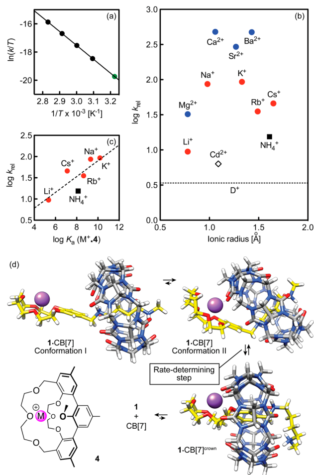
Figure 2. (a) Eyring plot describing the dethreading of axle 1 from [2]pseudorotaxane 1 •CB[7] at 50, 60, 70, and 80 °C (black dots); extrapolation to 37 °C (green dot). (b) Logarithmic plot of the dethreading rate constants k_{rel} as a function of the radius of the added cations; rates relative to the dethreading in the absence of cations. (c) Correlation between dethreading rate constants k_{rel} and the binding affinities of hemispherand 4 toward various cations in D 2 O-saturated chloroform- d . (d) A plausible “lubricated” dethreading pathway: cations (Na + , for example; violet sphere) stabilize intermediate 1 •CB[7] crown and the transition state leading to its formation, to a greater extent than [2]pseudorotaxane 1 •CB[7] (conformation II, and a fortiori, conformation I), thereby favoring CB[7] egression. CB[7] carbon atoms in gray, axle carbons in yellow. Structures optimized at the B97-D/SVP level; the second, likely inert benzo-15-crown-5 stopper of axle 1 has been replaced by a hydrogen atom, to limit the total number of conformations, and to shorten optimization time; solvent molecules omitted.
