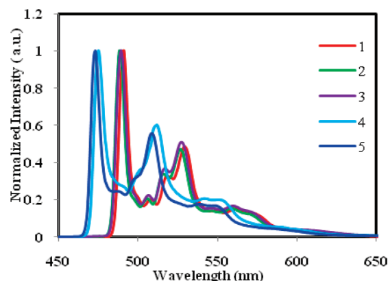
Figure 4. Normalized emission spectra of complex 1–5 in 2-methyltetrahydrofuran (77 K). \lambda_{\text{ex}} = 350 \text{ nm} .
