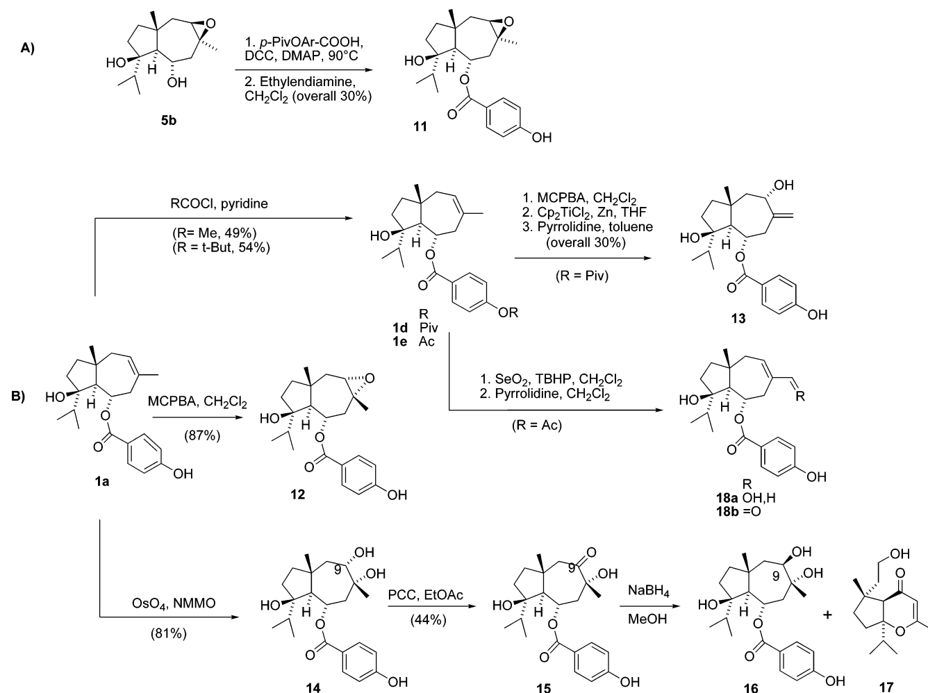
Scheme 3. Possible Mechanism for the Oxidative Fragmentation of the Daucean Core of 15 and the Formation of 17
