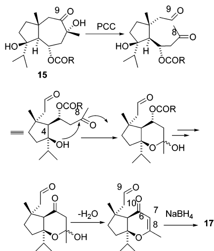
Scheme 3. Possible Mechanism for the Oxidative Fragmentation of the Daucean Core of 15 and the Formation of 17
