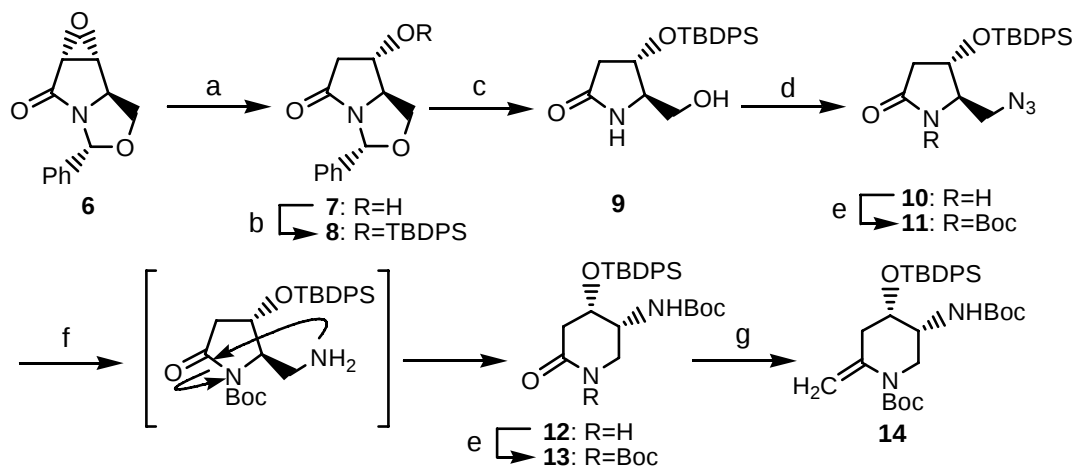
Scheme 2. Reagents and conditions: (a) (PhSe) 2 , NaBH 4 , AcOH, EtOH, rt, 86%; (b) TBDPS-Cl, Im, DMF, 0°C to rt; (c) H 2 NNH 2 -H 2 O, 10% Pd-C, MeOH, reflux, 86% (2 steps); (d) (i) MsCl, Et 3 N, CH 2 Cl 2 , 0°C; (ii) NaN 3 , DMF, 80°C; (e) Boc 2 O, 4-DMAP, CH 2 Cl 2 , rt, 88% (3 steps); (f) H 2 , 10% Pd-C, MeOH-H 2 O (12:1), 3 atm, rt, 92%; (g) Cp 2 TiMe 2 , toluene, 105°C, 78%.
