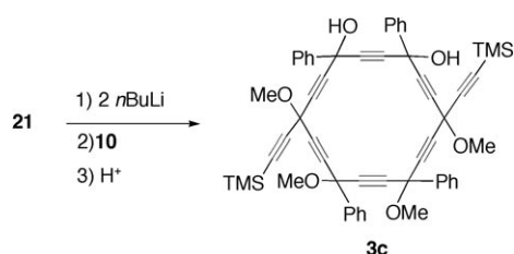
Scheme 12. Cyclization of a stereoisomeric mixture of the bis-terminal heptyayne tetraether 21 with dibenzoylacetylene ( 10 ) to the diethynyl[6]-pericyclinediol 3c .
