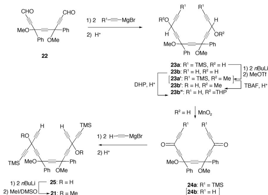
Scheme 11. Synthesis of bis-terminal carbinol-skipped heptyaynes 25 and 21 .
