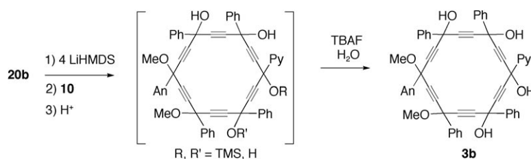
Scheme 10. Formation of a totally dissymmetric heteroaryl-substituted hexaoxy[6]pericycline 3b .
