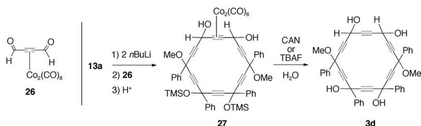
Scheme 13. Synthesis of a stable hexaoxy[6]pericyclyne 3d with adjacent secondary carbinol vertices using Gorgues' acetylenedicarbaldehyde cobalt complex 26 .
