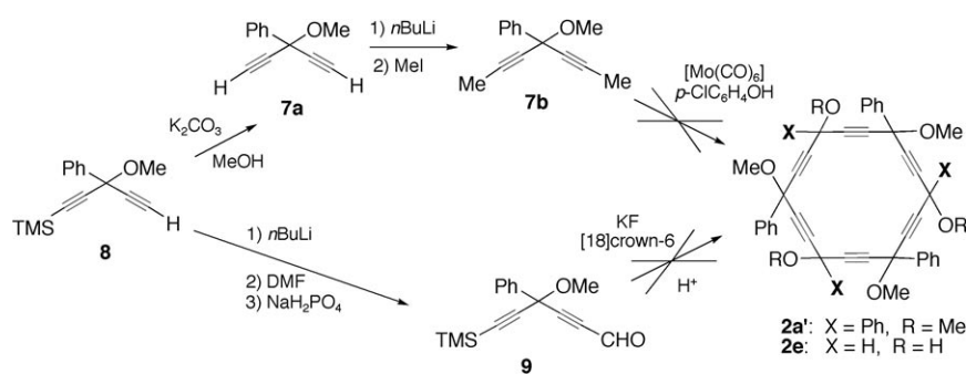
Scheme 3. Attempted sequential processes [ 6 \times 3 ] metathesis or [ 3 \times 6 ] alkynyl-oxopropargyl coupling) for the direct formation of symmetrical hexaoxy[6]pericyclines.
