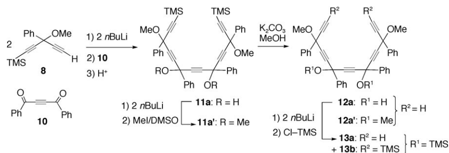
Scheme 5. Preparation of C_{14} tetraphenyltetraoxypentaynes.
