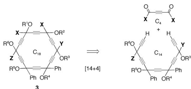
Scheme 4. General [14+4] strategy for the generation of hexaoxy[6]pericyclines of type 3.
