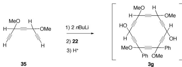
Scheme 19. Formation of hexaoxy[6]pericyclic 3g with four adjacent secondary carbinol vertices by [8+10] cyclization.
