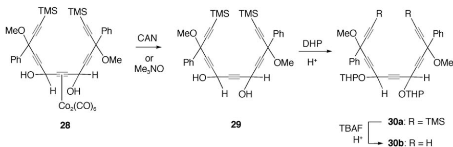
Scheme 14. Preparation of skipped C_{14} pentaynes containing two adjacent secondary carbinol vertices, with a view to a putative [14+4] cyclization with the C_4 dicarbonylacetylenes 10 or 26 .
