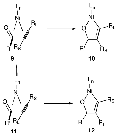
Scheme 1. Rationale of Regioselectivity
