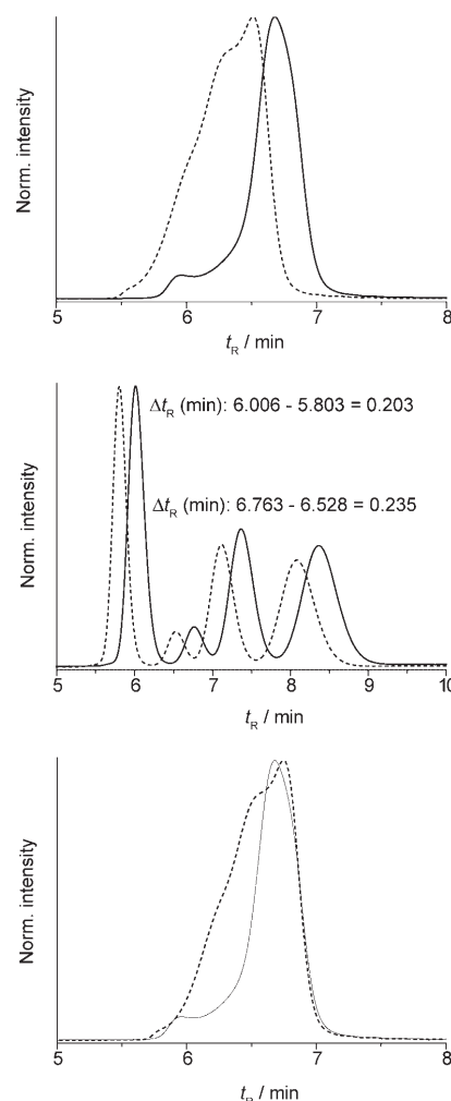
Figure 6. GPC chromatograms at 25°C (solid line) and 55°C (dashed line) of 3b uncorrected (top); PSMP (polystyrene) standard, M_w : 30 300, 10 150, 5 000 and 1 600 (middle); 3b with correction of PSMP M_w 10 150 (uncorrected curve of 3b + 0.235 minutes; bottom).
