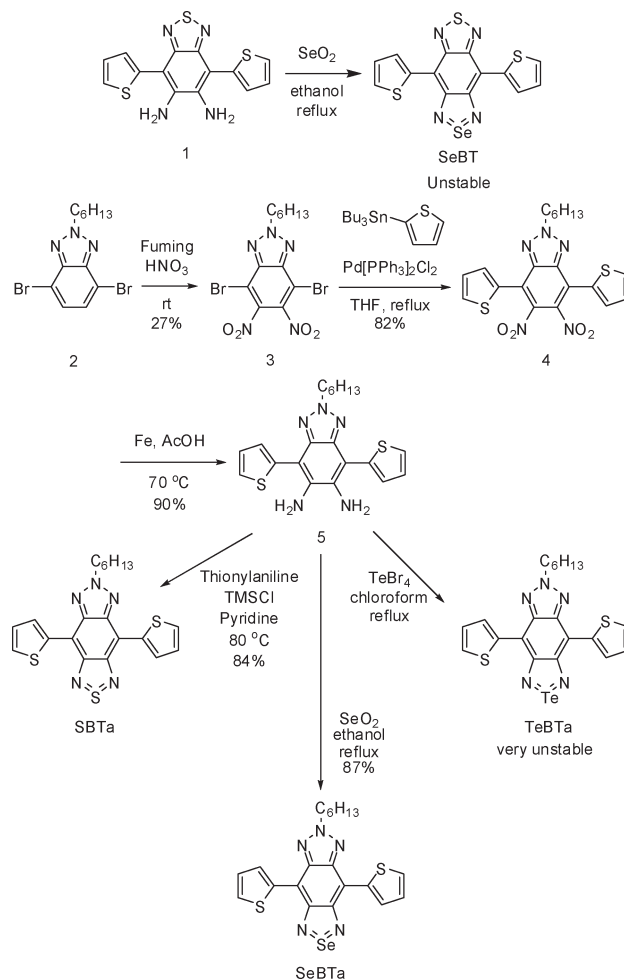
Scheme 1. Synthesis of SeBT, SBTa, SeBTa, and TeBTa
