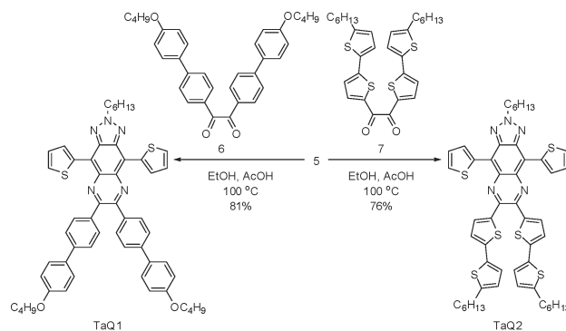
Scheme 2. Synthesis of TaQ1 and TaQ2
