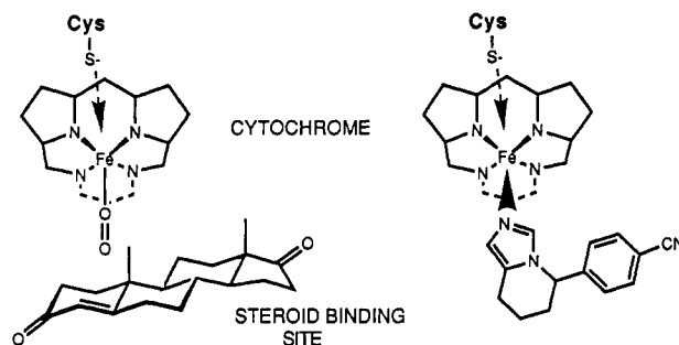
Figure 3. Proposed binding model of CGS 16949 A to the cytochrome P-450-aromatase complex.
