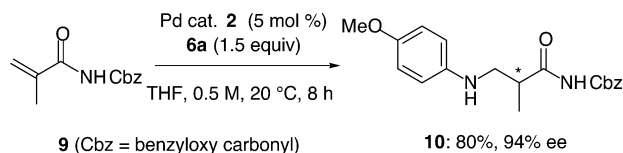
Scheme 4. Catalytic Asymmetric Protonation in the Conjugate Addition of Anisidine
