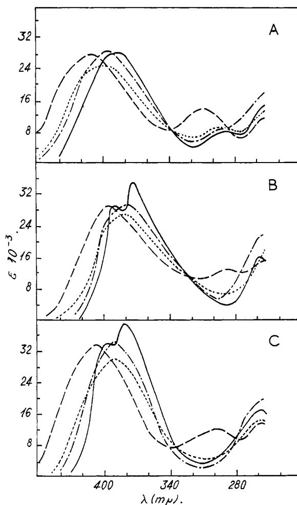
Fig. 4.—Azlactones (I) No. 48-59: A, R_1 = 3,4,5\text{-(CH}_3\text{O)}_3\text{-C}_6\text{H}_2\text{-} ; B, R_1 = 4\text{-CH}_2\text{COO-3-CH}_3\text{OC}_6\text{H}_3\text{-} ; C, R_1 = 3\text{-CH}_2\text{COO-4-CH}_2\text{OC}_6\text{H}_3\text{-} ; R_2 = \text{C}_6\text{H}_5\text{-} , —; R_2 = o\text{-NO}_2\text{C}_6\text{H}_4\text{-} , .....; R_2 = m\text{-NO}_2\text{C}_6\text{H}_4\text{-} , - · - · -; R_2 = p\text{-NO}_2\text{C}_6\text{H}_4\text{-} , - - - -.
