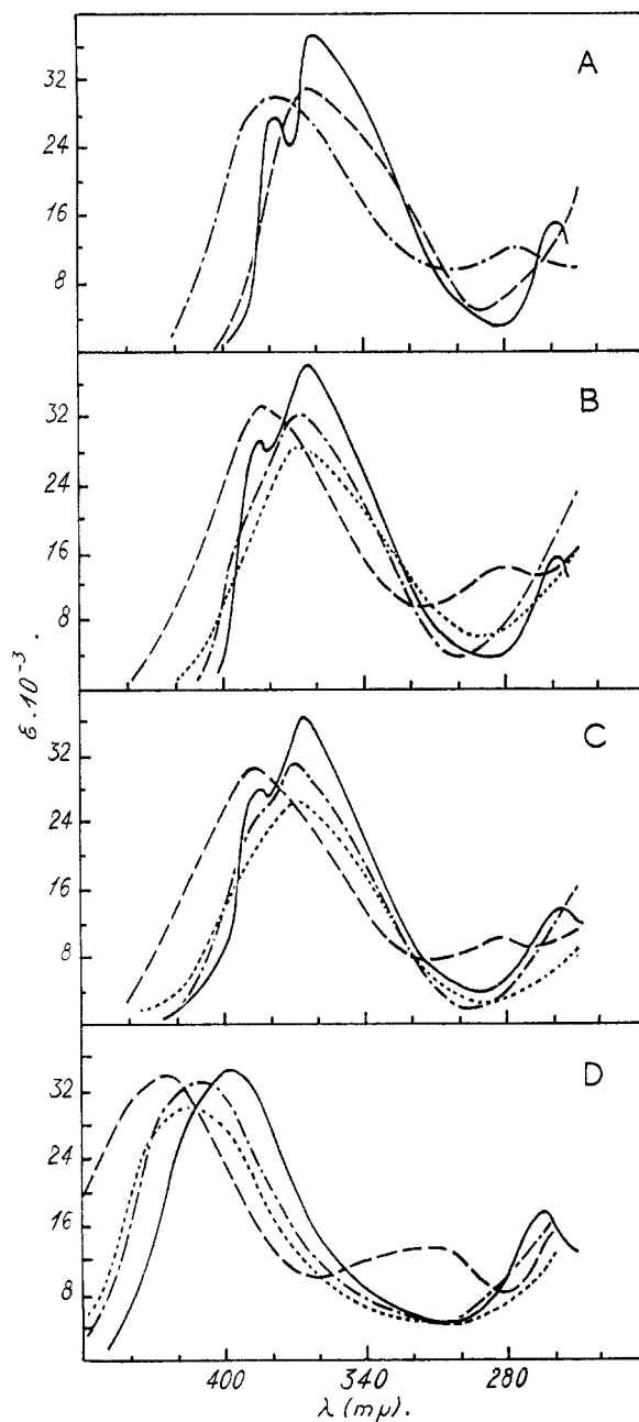
Fig. 2.—Azlactones (I) No. 17-31: A, R_1 = m-CH_3COOC_6H_4 ; B, R_1 = p-CH_3COOC_6H_4 ; C, R_1 = 2,3-(CH_3O)_2C_6H_3 ; D, R_1 = 3,4-(CH_3O)_2C_6H_3 , R_2 = C_6H_5 , —; R_2 = o-NO_2C_6H_4 , .....; R_2 = m-NO_2C_6H_4 , - - - - -; R_2 = p-NO_2C_6H_4 , - · - · -.
