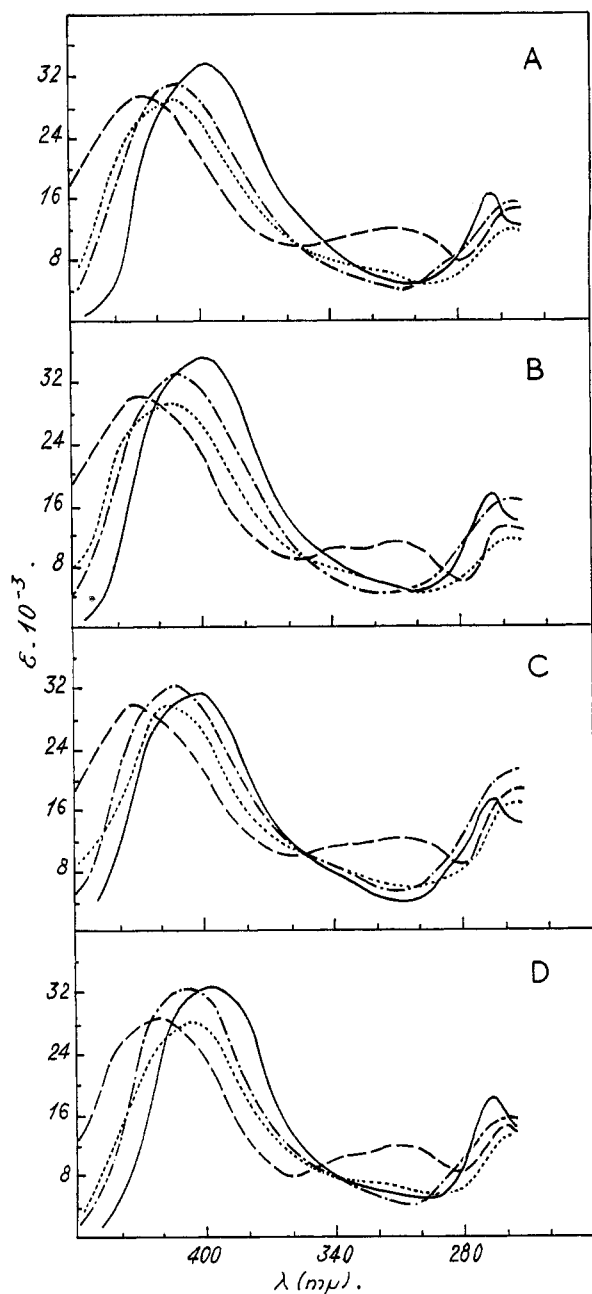
Fig. 3.—Azlactones (I) No. 32-47: A, R_1 = 3\text{-C}_2\text{H}_5\text{O-4-CH}_3\text{OC}_6\text{H}_3\text{-} ; B, R_2 = 4\text{-C}_2\text{H}_5\text{O-3-CH}_3\text{OC}_6\text{H}_3\text{-} ; C, R_1 = 3,4\text{-(C}_2\text{H}_5\text{O)}_2\text{C}_6\text{H}_3\text{-} ; D, R_1 = 3,4\text{-CH}_2\text{O}_2\text{C}_6\text{H}_3\text{-} , R_2 = \text{C}_6\text{H}_5\text{-} , —; R_2 = o\text{-NO}_2\text{C}_6\text{H}_4\text{-} , .....; R_2 = m\text{-NO}_2\text{C}_6\text{H}_4\text{-} , - · - · -; R_2 = p\text{-NO}_2\text{C}_6\text{H}_4\text{-} , - - - -.
