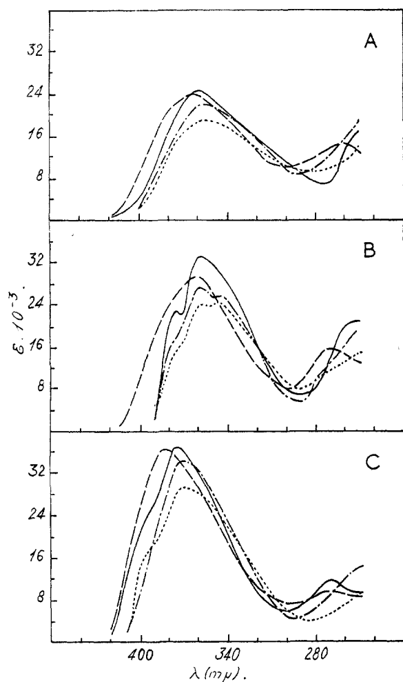
Fig. 5.—Azlactones (I) No. 60–71: A, R_1 = o\text{-NO}_2\text{C}_6\text{H}_4\text{-} ; B, R_1 = m\text{-NO}_2\text{C}_6\text{H}_4\text{-} ; C, R_1 = p\text{-NO}_2\text{C}_6\text{H}_4\text{-} ; R_2 = \text{C}_6\text{H}_5\text{-} , —; R_2 = o\text{-NO}_2\text{C}_6\text{H}_4\text{-} , .....; R_2 = m\text{-NO}_2\text{C}_6\text{H}_4\text{-} , - - - - -; R_2 = p\text{-NO}_2\text{C}_6\text{H}_4\text{-} , - · - · - ·.
