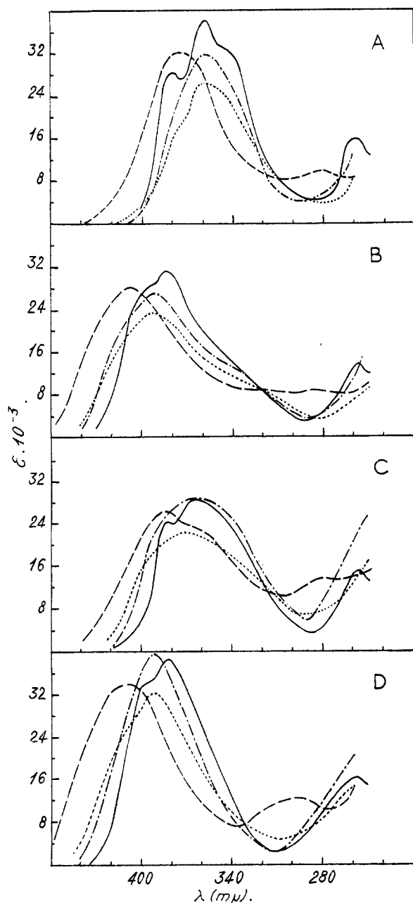
Fig. 1.—Azlactones (I) No. 1-16: A, R_1 = C_6H_5 ; B, R_1 = o-CH_3OC_6H_4 ; C, R_1 = m-CH_3OC_6H_4 ; D, R_1 = CH_3OC_6H_4 , R_2 = C_6H_5 , —; R_2 = o-NO_2C_6H_4 , .....; R_2 = m-NO_2C_6H_4 , - - - - -; R_2 = p-NO_2C_6H_4 , - · - · -.
