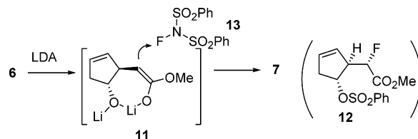
SCHEME 3. Diastereoselective Fluorination of 6
