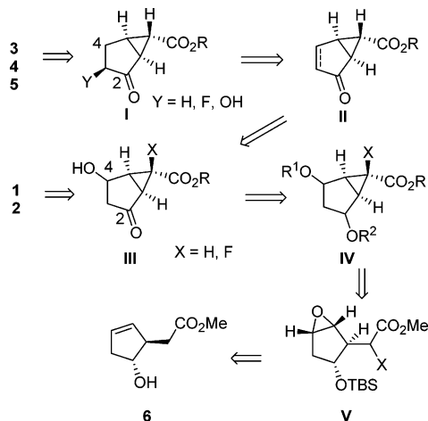
SCHEME 1. Synthetic Plan for mGluR2/3 Agonists 1–5
