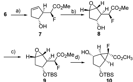
SCHEME 2. Stereoselective Preparation of 10 (IV: X = F) a
