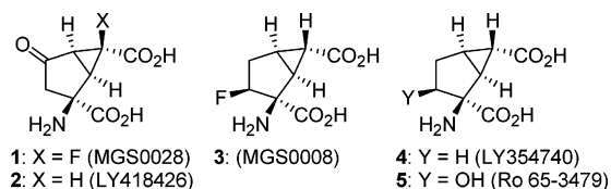
FIGURE 1. Highly selective and potent mGluR2/3 agonists.
