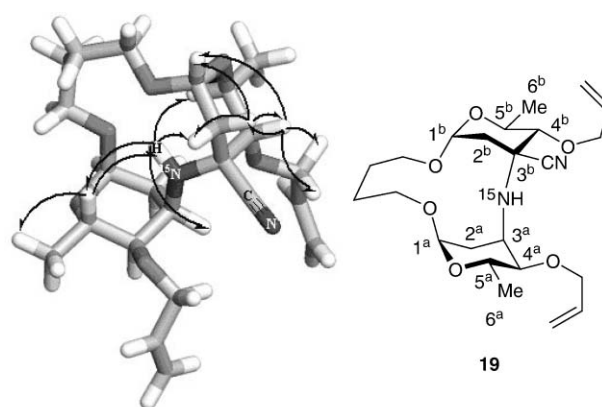
Fig. 2 Calculated structure and main NOE connectivities of aminocyanide 19 (these connectivities are also depicted in the graphic created by a molecular modelling study): 5- \text{H}^a (6- \text{H}^a , ^{15}\text{NH} ), ^{15}\text{NH} (5- \text{H}^a , 3- \text{H}^a , 2- \text{H}^b_{\text{eq}} , 5- \text{H}^b ), 2- \text{H}^b_{\text{ax}} (2- \text{H}^b_{\text{eq}} , 1- \text{H}^b , 4- \text{H}^b ), 4- \text{H}^b (1- \text{H}^b , 2- \text{H}^b , -\text{O}-\text{CH}_2-\text{CH}=\text{CH}_2 ).
