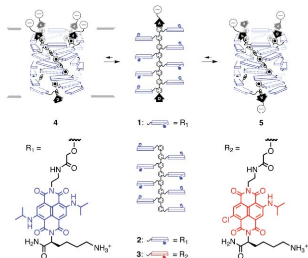
Fig. 1 Notional self-assembly of the blue, asymmetric push–pull rod 1 into parallel \pi -helix 4 in lipid bilayer membranes and antiparallel \pi -helix 5 in solution; for \pi -donor D and \pi -acceptor A with anionic anchor, please see Scheme 1. The symmetric blue and red controls 2 and 3 have been described. 18–20
