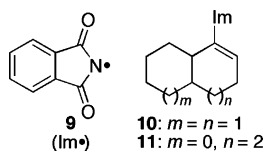
FIGURE 1. Reaction of imidyl radicals 9 with cyclodecyne leads to imidyl-substituted bicyclic alkenes 10 and 11 through a radical addition/cyclization sequence.
