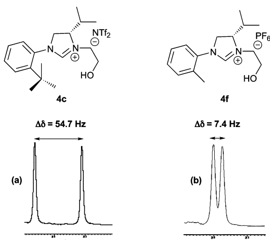
Fig. 2 Influence of the aryl substituent on the chiral discrimination: ^1\text{H} spectra (400 MHz, \text{CD}_2\text{Cl}_2 ) of ( rac )-Mosher salt 5 in imidazolinium 4c (a) and 4f (b) in presence of crown ether 18C6.
