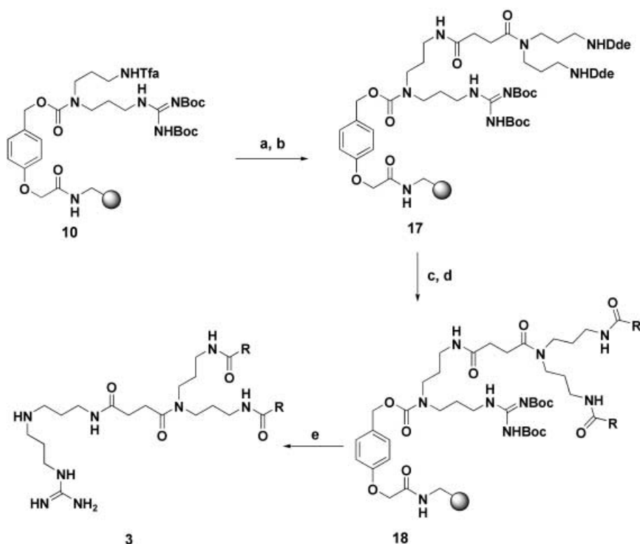
Scheme 5. Reagents and conditions: a) 1 M KOH/THF/MeOH (4:3:1), 2 h; b) acid 13 (1.7 equiv), DIC (2 equiv), HOBT (2 equiv), CH 2 Cl 2 , 2 h; c) hydrazine/DMF (5 %), d) carboxylic acids (4 equiv), DIC (4 equiv), HOBT (4 equiv), CH 2 Cl 2 , 2 h; e) TFA/CH 2 Cl 2 /H 2 O/thioanisole (8:0.5:0.5:1), 2 h.
