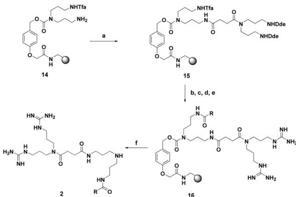
Scheme 4. Reagents and conditions: a) Acid 13 (2 equiv), DIC (2 equiv), HOBT (2 equiv), CH 2 Cl 2 , DMAP (0.1 equiv), 2 h; b) hydrazine/DMF (5 %), 2 h; c) N,N' -bis( tert -butoxycarbonyl)- S -methylisothiourea (4 equiv), pyridine, THF, 2 h; d) 1 M KOH/THF/MeOH (4:3:1), 2 h; e) carboxylic acids (4 equiv), DIC (4 equiv), HOBT (4 equiv), CH 2 Cl 2 , 2 h; f) TFA/CH 2 Cl 2 /H 2 O/thioanisole (8:0.5:0.5:1), 2 h.
