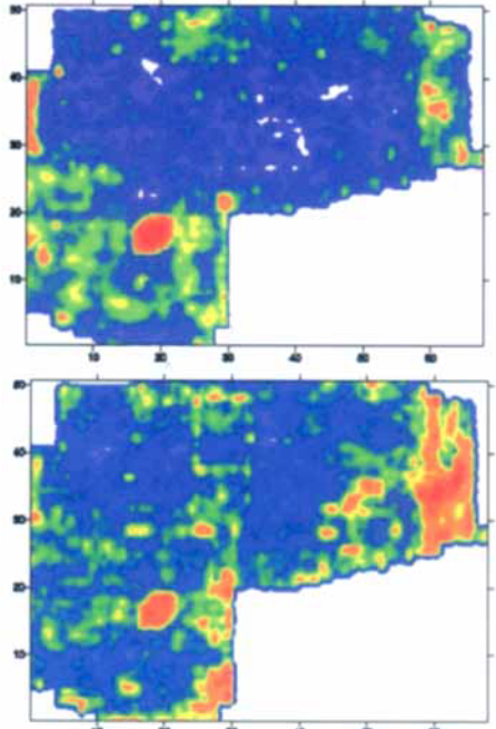
FIGURE 2. GPR amplitude slices from 25–50 cm depth (upper map) and 50–75 cm (lower) in Grid 1. Blue colours are very low-amplitude reflections, indicating open areas. Red areas are high-amplitude reflections, indicating the presence of buried stone architecture. The northern structure, mapped more precisely in Grid 2, can be seen in the lower slice at the centre top of the map.
