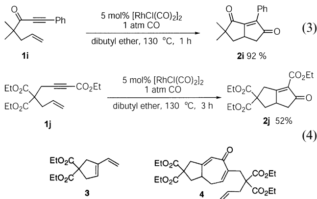
Fig. 1. By-products from enyne 1c .
