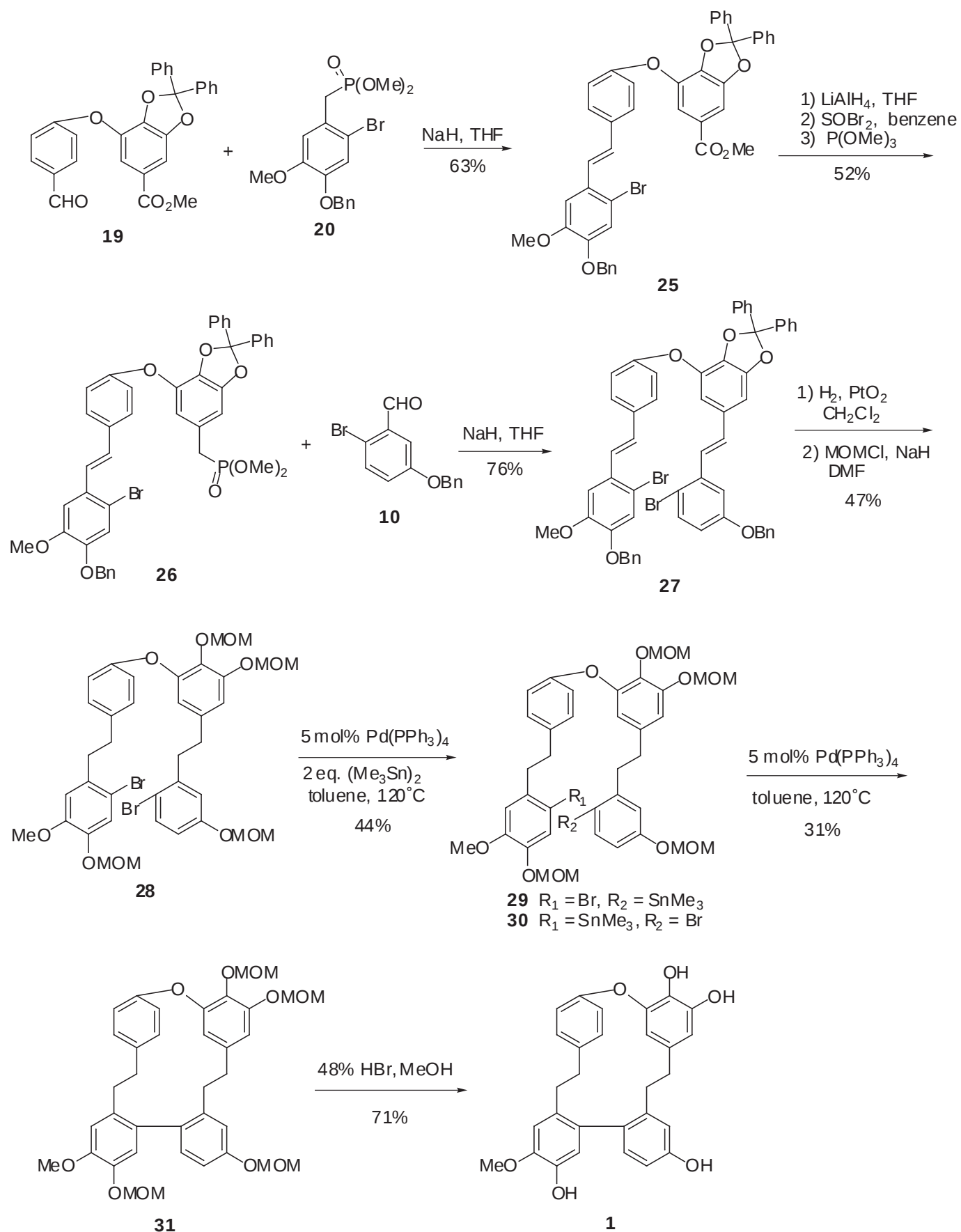
Scheme 4 Synthesis of plagiocchin A ( 1 )
