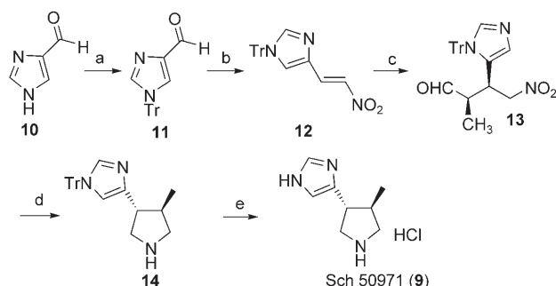
Scheme 2. Total synthesis of Sch 50971 ( 9 ). Conditions: a) TrCl, TEA, CH_2Cl_2 , RT, 14 h, 95%; b) CH_3NO_2 , piperidine, AcOH, RT, 8 h, 79%; c) propionaldehyde, iPrOH/CH_2Cl_2 (v/v 1:1) 20 mol % 1 , 0°C, 24 h, 99% ee, 20:1 d.r., 78%; d) 20% Pd(OH) 2 , MeOH, 45 psi, RT, 96 h, 65%; e) 95% TFA, 3 h, 91%.
