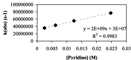
Figure 20. A plot of the observed rate constant of transient decay (380 nm) versus concentration of pyridine produced by LFP (308 nm) of 1c in carbon tetrachloride.
