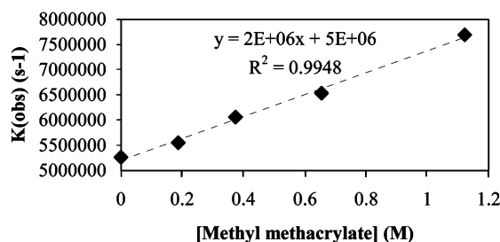
Figure 16. A plot of the observed rate constant of transient decay (406 nm) versus the concentration of methyl methacrylate produced by LFP (308 nm) of 1b in cyclohexane containing 0.247 M of pyridine.
