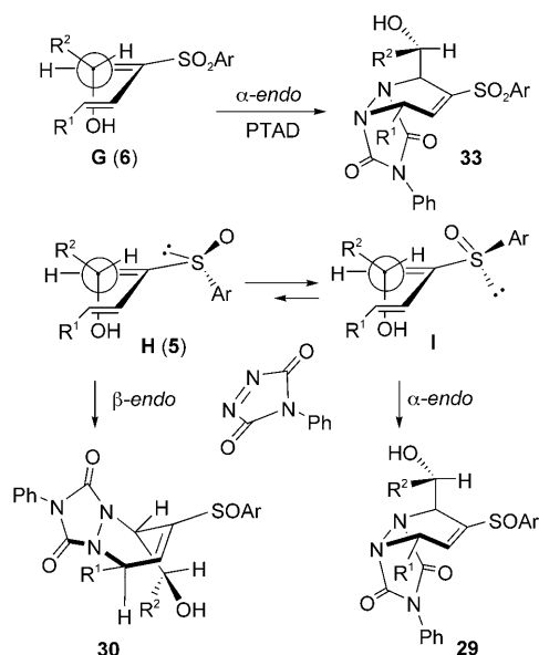
Scheme 6. Stereochemical rationalization for ( Z,E )-sulfinyl and -sulfonyl-dienes.
