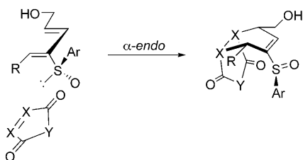
Scheme 4. Stereochemical rationalization for 3-sulfinyldienes.
