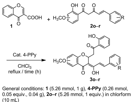
Scheme 4. Michael addition of 1,3-dicarbonyl 2o-r on acid 1 .
