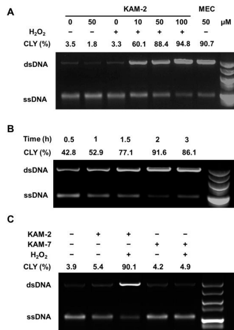
Fig. 5 DNA interstrand cross-linking (ICL) ability of KAM-2 . (A) Denaturing alkaline agarose gel electrophoresis performed with 1 μg linearized pBR322 plasmid DNA and indicated concentrations of KAM-2 or MEC with or without H 2 O 2 (10 mM) for 2 h at 37 °C. (B) Denaturing alkaline agarose gel electrophoresis performed with 1 μg linearized pBR322 plasmid DNA, 50 μM KAM-2 , and 10 mM H 2 O 2 at 37 °C for indicated time. (C) Denaturing alkaline agarose gel electrophoresis performed with 1 μg pBR322, 50 μM KAM-2 or KAM-7 with or without H 2 O 2 (10 mM) for 2 h at 37 °C. CLY: cross-linking yield.
