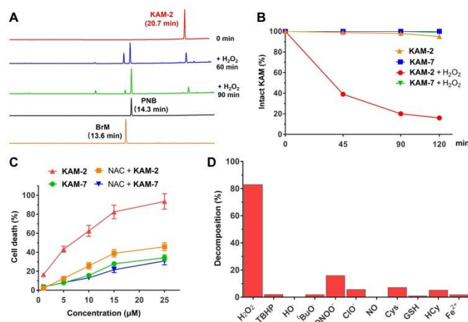
Fig. 2 \text{H}_2\text{O}_2 -responsive behaviours of KAM-2 . (A) Decomposition of 100 \mu\text{M} KAM-2 in presence of \text{H}_2\text{O}_2 (2 eq.) as monitored by RP-HPLC (254 nm). (B) Decomposition of KAM-2 and KAM-7 (100 \mu\text{M} ) with or without \text{H}_2\text{O}_2 (10 eq.). (C) The effects of NAC on the cytotoxicity of KAM-2 and KAM-7 in HL-60 cells after 72 h incubation. (D) Selectivity of KAM-2 toward \text{H}_2\text{O}_2 as determined by measuring its decomposition ratios under various stimuli.
