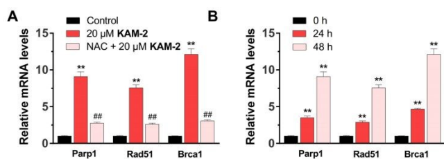
Fig. 9 The effects of 20 \mu\text{M} KAM-2 on the expression DDR-related mRNA levels tested by real-time PCR. Mean \pm SD, n = 3 . ** p < 0.01 vs. control or 0 h treatment; ## p < 0.01 vs. 20 \mu\text{M} KAM-2 treatment.
