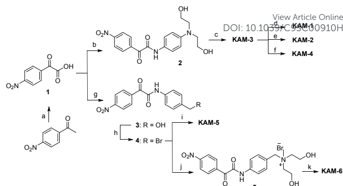
Scheme 2. Synthesis of KAM prodrugs. Reactants and conditions: a) \text{SeO}_2 , pyridine, 90 °C, \text{N}_2 , 35%; b) N -4-aminophenyl diethanolamine, EDCI, DIEA, DMF, 42%; c) \text{MsCl} , DMAP, TEA, DCM, reflux, 70%; d) \text{LiCl} (5 eq.), DMF, 60 °C, 65%; e) \text{NaBr} (5 eq.), DMF, 60 °C, 67%; f) \text{LiCl} (1 eq.), MeCN, 60 °C, 23%; g) (4-aminophenyl)methanol, EDCI, DIEA, DMF, 33%; h) \text{CBr}_4 , \text{PPh}_3 , DCM, 0 °C–r.t., 50%; i) N -(4- \text{N}' , \text{N}' -dimethylaminophenyl)-bis(2-chloroethyl)amine, MeCN, 43%; j) N -methyl-diethanolamine, \text{CHCl}_3 , reflux, 76%; k) \text{SOCl}_2 , r.t., 62%.
