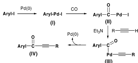
FIGURE 1. Possible Explanation for Carbonylative Coupling Reactions.
