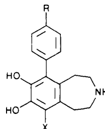
3a, R = H; X = H b, R = H; X = Cl c, R = OH; X = H d, R = OH; X = Cl
