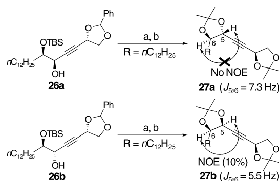
Scheme 6. Synthesis of acetals 27a and 27b . a) TBAF, THF, RT; b) Me 2 C(OMe) 2 , p TsOH · H 2 O, CH 2 Cl 2 , RT, 94 % over 2 steps from 26a , 97 % over 2 steps from 26b . TBAF = tetrabutylammonium fluoride, p Ts = 4-toluenesulfonyl = tosyl.
