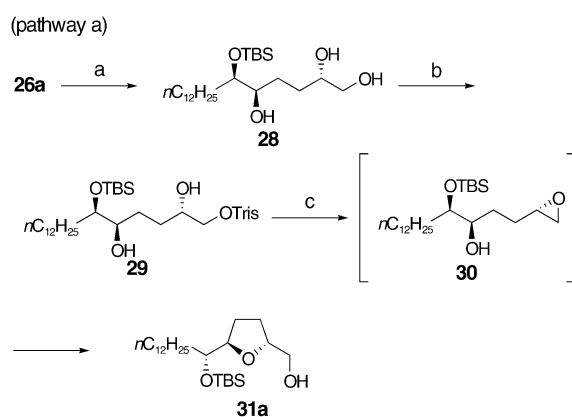
Scheme 7. Synthesis of THF-ring moiety 31a . a) H 2 , 10 % Pd/C, EtOAc, RT, 94 %; b) TrisCl, pyridine, CH 2 Cl 2 , 0 °C → RT, 87 %; c) K 2 CO 3 , MeOH, 0 °C → RT, 70 %. Tris = 2,4,6-triisopropylbenzenesulfonyl.
