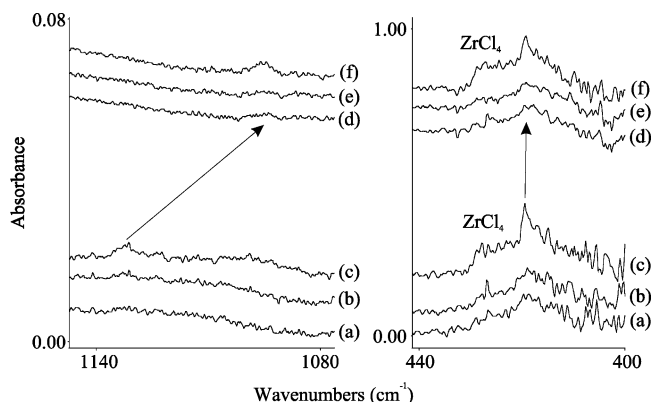
Figure 4. IR spectra in the 1140–1080 and 440–400 \text{cm}^{-1} regions of the spectra taken after (a) laser-ablated zirconium atoms were reacted with 0.5% \text{CCl}_4/\text{Ar} , (b) the matrix sample was irradiated at \lambda > 290 nm and (c) at \lambda > 220 nm, and after (d) zirconium atoms were reacted with 0.5% ^{13}\text{CCl}_4/\text{Ar} (90% ^{13}\text{C} enriched), (e) the matrix sample was irradiated at \lambda > 290 nm and (f) at \lambda > 220 nm. The product absorptions are marked with arrows.
