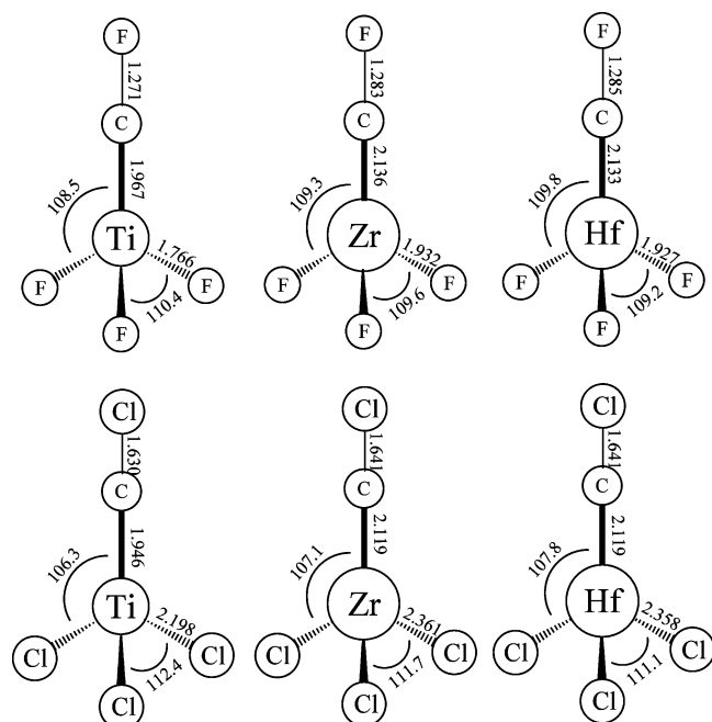
Figure 3. Optimized geometries of the \text{FC}\div\text{MF}_3 and \text{ClC}\div\text{MCl}_3 complexes computed with \text{C}_{3v} symmetry at the B3LYP//6-311+G-(2d)/SDD level of theory. Bond lengths are in angstroms and angles are in degrees.
