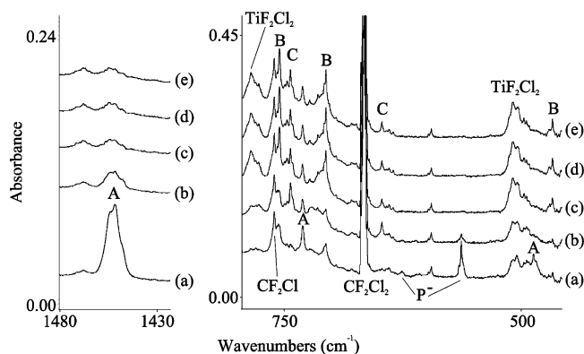
Figure 5. Infrared spectra in the 1480–1425 and 800–450 \text{cm}^{-1} regions taken after (a) laser-ablated titanium atoms were reacted with 1.0% \text{CF}_2\text{Cl}_2/\text{Ar} during condensation at 8 K for 1 h, and the resulting matrix was subjected to (b) irradiation with light \lambda > 290 nm, (c) irradiation with \lambda > 220 nm, (d) annealing to 30 K, and (e) irradiation with \lambda > 470 nm. Product absorptions labeled A belong to the \text{FC}\div\text{TiFCl}_2 complex, B peaks are assigned to the \text{ClC}\div\text{TiF}_2\text{Cl} species, and the identity of C peaks is not resolved. Common precursor products \text{CF}_2\text{Cl} radical and parent anion ( \text{P}^- ) are labeled in the figure; see ref 15.
