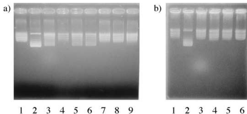
Fig. 1. Cleavage of supercoiled pGEM9zf(-) DNA by topoisomerase I in the presence of 2-[2-(2-alkynylphenyl)ethynyl]benzonitriles 7–10 , 1,4-bis(dec-3-ene-1,5-diynyl)benzene ( 11 ), and 4,4'-bis(dec-3-ene-1,5-diynyl)-1,1'-biphenyl ( 12 )
