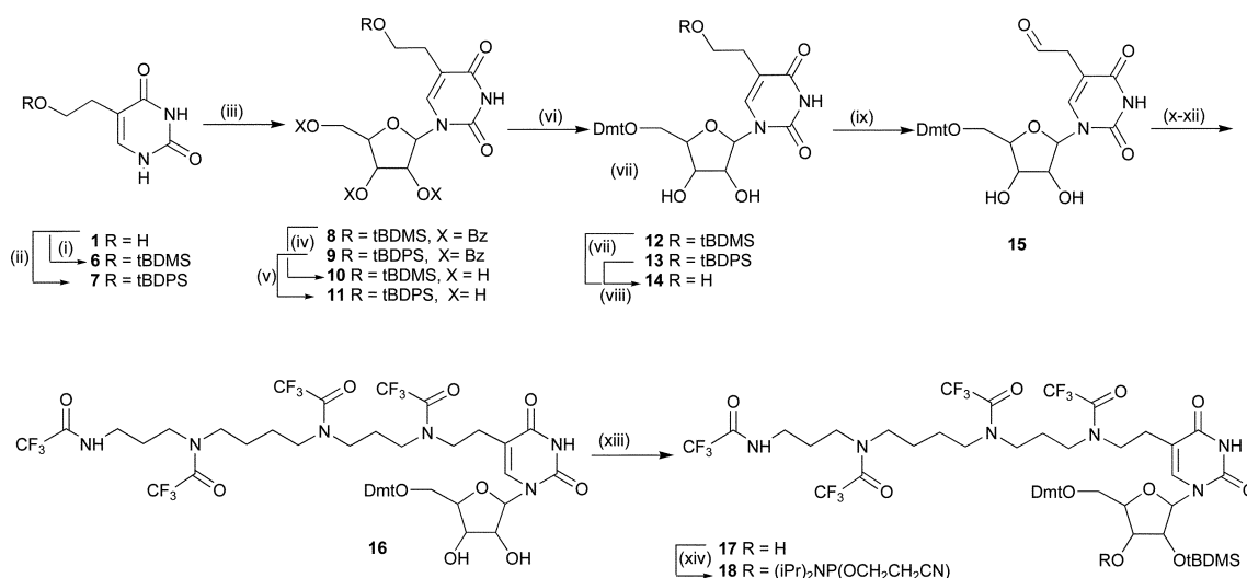
Scheme 2 Synthesis of the phosphoramidite monomer of the uridine-spermine conjugate ( 18 ). Reagents and conditions: (i) \text{tBDMSCl} , imidazole, DMF, room temperature, 98%; (ii) \text{tBDPSCl} , imidazole, DMF, room temperature, 99%; (iii) either 6 or 7 , 1- O -acetyl-2,3,5-tri- O -benzoyl- \beta -D-ribofuranose, TMSCl, hexamethyldisilazane, \text{SnCl}_4 , MeCN, room temperature, 68% from 6 , 60% from 7 ; (iv) \text{NH}_3 (MeOH), room temperature, 82%; (v) \text{NH}_3 (MeOH), room temperature, 72%; (vi) either 10 or 11 , DmtCl, pyridine, room temperature, 74% from 10 , 70% from 11 ; (vii) TBAF, THF, room temperature, 98%; (viii) TBAF, THF, room temperature, 75%; (ix) Swern procedure 14 , oxalyl chloride, DMSO, TEA, DCM, -60^\circ\text{C} , 61%; Moffat procedure 14 , DMSO, pyridine, trifluoroacetic acid, room temperature, 42%; (x) spermine, pyridine, methanol, room temperature; (xi) same pot \text{NaBH}_4 ; (xii) trifluoroacetic anhydride, pyridine, room temperature, 57% (three steps); (xiii) \text{tBDMSCl} , \text{AgNO}_3 , pyridine, THF, room temperature, 69%; (xiv) 17 , 2-cyanoethyl- N -diisopropylamine chlorophosphoramidite, diisopropylamine, DCM, room temperature, 86%.
