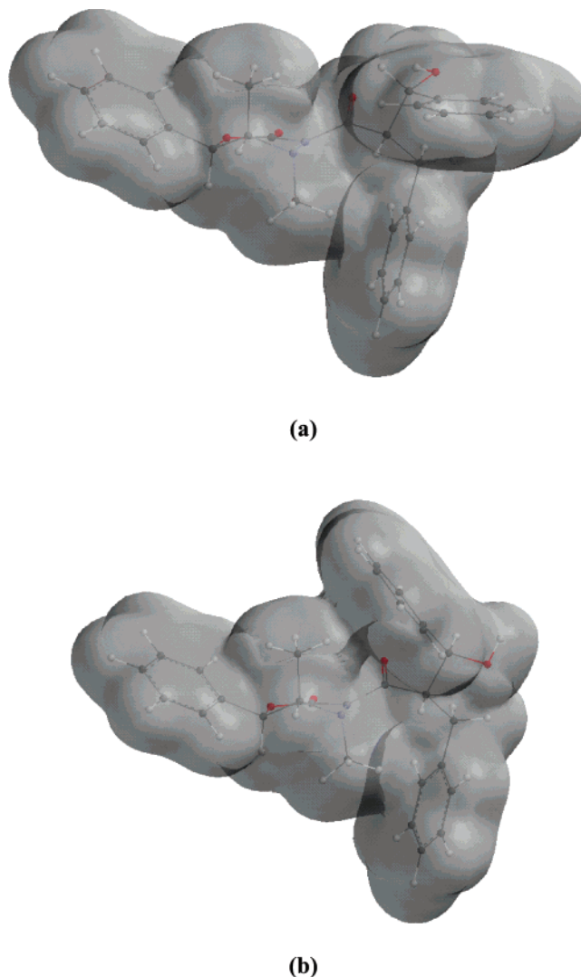
FIGURE 8. Isodensity surfaces of the optimized geometry of (a) conformer 1 and (b) conformer 2 of oxadiazinone 5a obtained using the AM1 semiempirical method. The isodensity surface is plotted at a value of 0.002.
