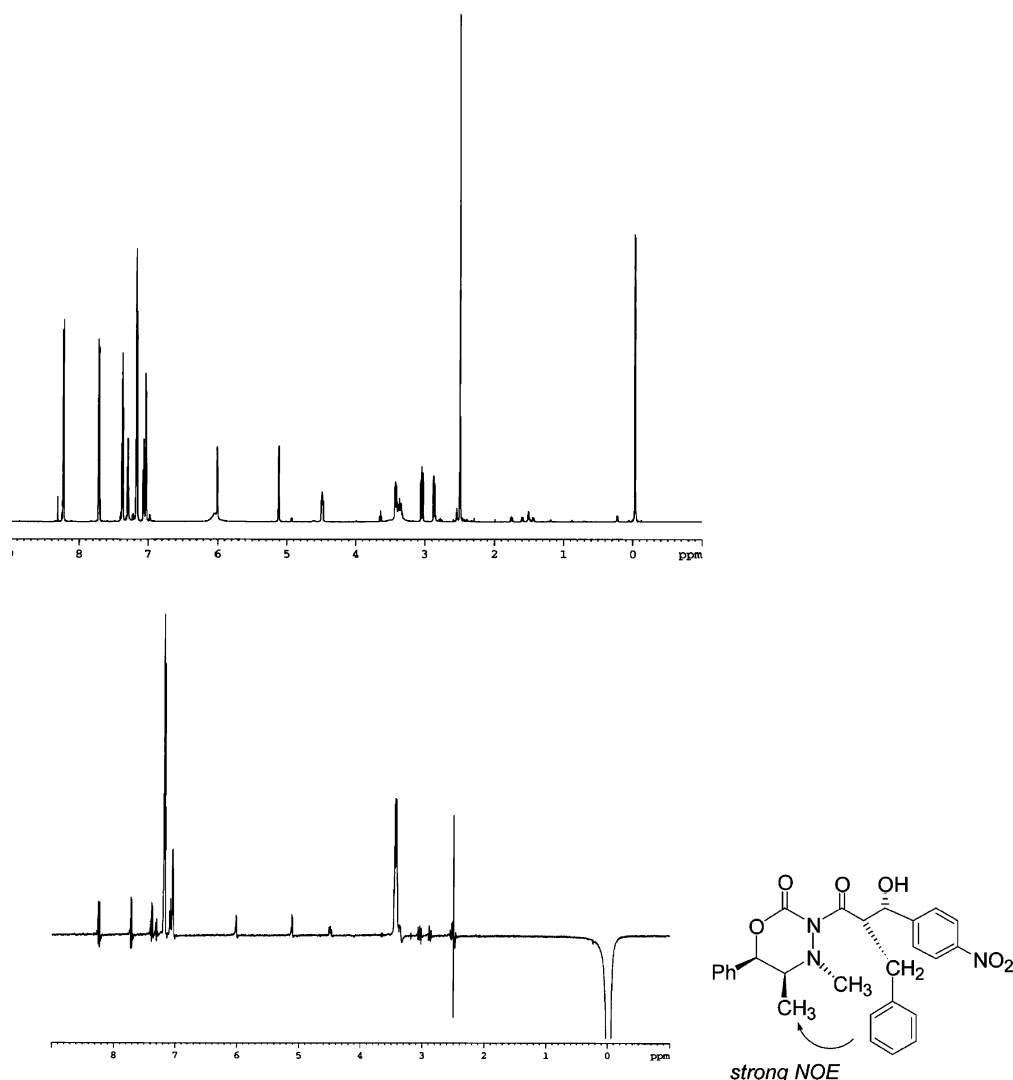
FIGURE 5. NMR spectrum of oxadiazinone 5e . (a) 700 MHz 1 H NMR spectrum of 5e in DMSO- d 6 . (b) 500 MHz 1 H NMR NOEDIFF spectrum of 5e in DMSO- d 6 .
