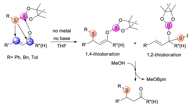
Scheme 1. Postulated Substrate-Reagent Interaction To Promote 1,4- and 1,2-Thioboration and Protic Work-up Step towards \beta -Sulfido Carbonyl Compounds
