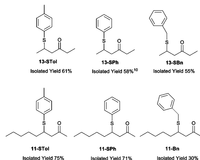
Figure 5. Comparative study of thioboration/protonation with thiodioxaborolanes PhS-Bpin ( 1 ), BnS-Bpin ( 12a ), and TolS-Bpin ( 12b ).
