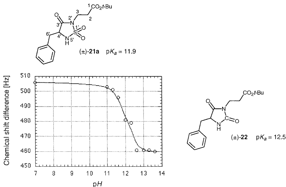
Fig. 3. ^1\text{H} -NMR Titration to determine the pK_a value of (±)-21a. The chemical shift difference between the signal of H-C(6') and the t -Bu group is plotted against pH. Shown is also hydantoin analog (±)-22, for which the pK_a value was also determined by ^1\text{H} -NMR titration (not shown) [39].
