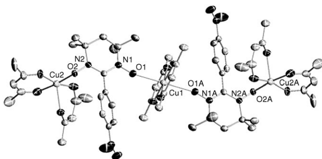
Figure 2. Molecular structure of 19 [(\text{Cu}(\text{hfac})_2)_3 \cdot (\mathbf{8d})_2] . F and H atoms are not represented. Thermal ellipsoids are drawn at the 30% probability level.
