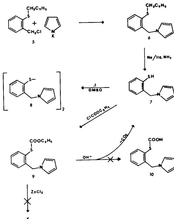
SCHEME I
