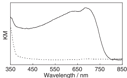
Figure 1. Diffuse reflectance UV-vis spectra of 4,4'-butadiynebenzylammonium disorbate before and after polymerization. Dotted line: monomer, solid line: after UV irradiation for 8 h.
