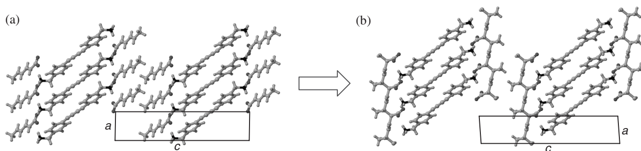
Figure 2. Crystal structure of 4,4'-butadienyldibenzylammonium disorbate viewed from crystallographic b axis. (a) Monomer recrystallized from methanol, (b) after X-ray irradiation for 48 h (Mo K\alpha , 40 kV, 200 mA).
