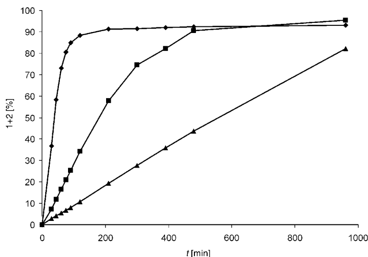
Figure 2. Catalyst performance of complex 8 at 50, 70 and 90°C; ♦: 90°C, ■: 70°C, ▲: 50°C.
