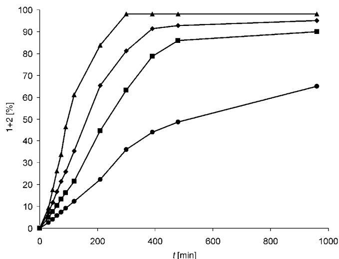
Figure 3. Activity of complexes 8–11 at 70°C; ♦: complex 8 ; ■: complex 9 ; ▲: complex 10 ; ●: complex 11 .
