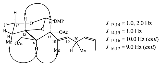
Fig. 2. NOESY Correlations and Vicinal Coupling Constants ( J_{\text{H-H}} ) of the Olefin, Prepared from 25
