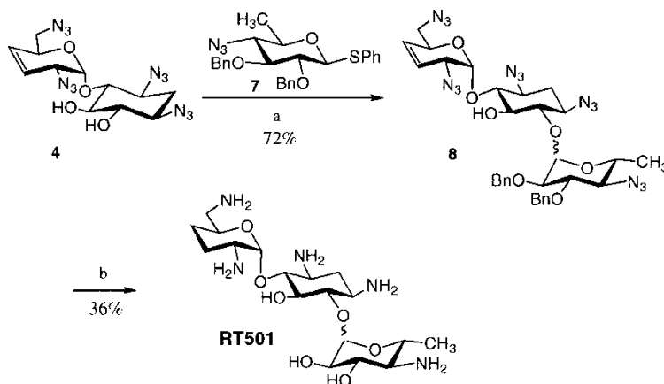
Scheme 2: Synthesis of 3',4'-dideoxy kanamycin B analog. Conditions: (a) NIS, TfOH, \text{Et}_2\text{O}:\text{CH}_2\text{Cl}_2 (3:1), (b) (i) \text{PMe}_3 , NaOH, THF, (ii) \text{Pd}(\text{OH})_2/\text{C} , HOAc, \text{H}_2\text{O} , (iii) Dowex 1X8-200 ( \text{Cl}^- form).
