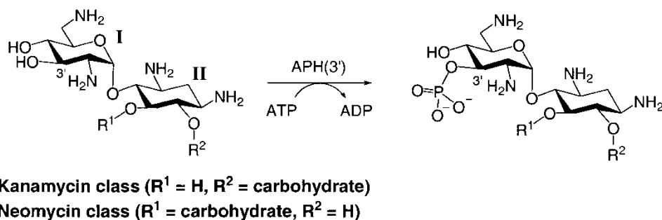
Figure 1: Phosphorylation of kanamycin and neomycin classes aminoglycosides by APH(3').
