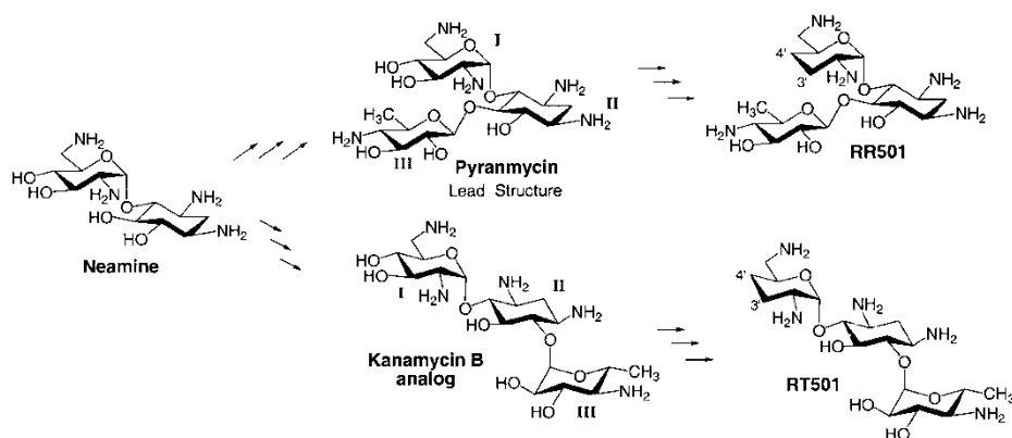
Figure 3: Proposed strategy for the synthesis of aminoglycoside with 3',4'-dideoxygenation.
