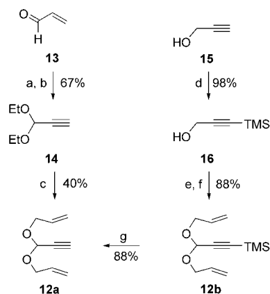
Scheme 4. Synthesis of the precursors of the Pauson–Khand reaction, 12a and 12b . a) \text{Br}_2 , 0–5 °C; then \text{HC}(\text{OEt})_3 , EtOH, RT, 99%; b) KOH (excess), [\text{Oct}_4\text{N}^+\text{Br}^-] (cat.), CyHex, reflux, 67%; c) allyl-OH (excess), TsOH (cat.), \text{C}_6\text{H}_6 (azeotropic removal of EtOH), 40%; d) n\text{BuLi} (2.3 equiv), THF/ n -hexane, –78 °C → RT, 4 h; then TMSCl (2.3 equiv), –78 °C → RT, 18 h; then aq. HCl (1.3 equiv), RT, 1 h, 98%; e) PCC (1.5 equiv), \text{CH}_2\text{Cl}_2 , RT, 3 h; f) allyl-OH (excess), TsOH (cat.), \text{C}_6\text{H}_6 , \Delta , 15 h, 88% over 2 steps; g) TBAF (1 equiv) in THF, \text{H}_2\text{O} /allyl-OH (2:1), RT, 1 h, 88%. CyHex = cyclohexane, Oct = octyl, PCC = pyridinium chlorochromate, TBAF = tetrabutylammonium fluoride, THF = tetrahydrofuran, TMS = trimethylsilyl, Ts = toluene-4-sulfonyl.
