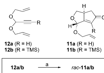
Scheme 5. Preparation of bicyclic intermediates of type 11 by the Pauson–Khand reaction. Optimized conditions: a) [\text{Co}_2(\text{CO})_8] (1.1 equiv), \text{CH}_2\text{Cl}_2 , molecular sieves (4 Å, 8 equiv by weight), RT, 2 h; then TMANO (8.8 equiv), air, 0 °C → RT, 15 h. For yields, see Table 1.
