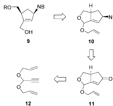
Scheme 3. Retrosynthetic analysis for CNAs of type 9 . NB=nucleobase.
