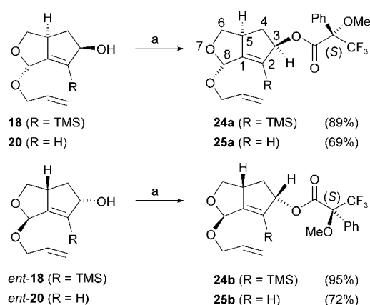
Scheme 12. Preparation of the Mosher (MTPA) esters from alcohols 18 , ent-18 , 20 , and ent-20 . a) ( S )-MTPA (1.1 equiv), DCC (1.1 equiv), DMAP (12 mol %), \text{CH}_2\text{Cl}_2 , 0^\circ\text{C} \rightarrow \text{RT} , 16 h.
