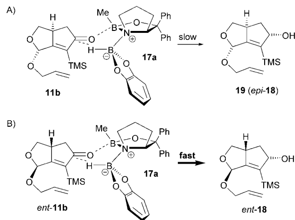
Scheme 8. Two competing transition structures in the kinetic resolution of rac - 11b by CBS reduction with catalyst 17a . Catalyst control is assumed: A) mismatched case (violation of substrate preference); B) matched case.
