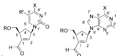
Scheme 16. Numbering used for compounds of type 23 , NB = various nucleobases.
