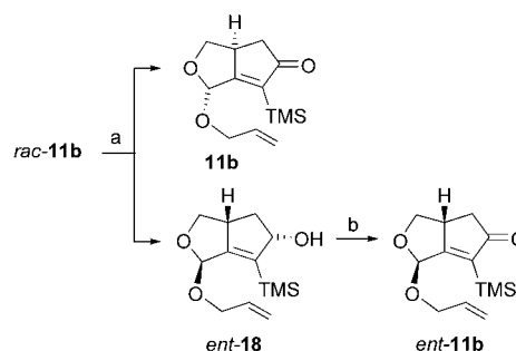
Scheme 7. Preparation of enantiomerically pure 11b and ent - 11b through kinetic resolution of the ketone rac - 11b by means of a CBS reduction. a) 17a (20 mol %), CB (0.85 equiv), THF/toluene, -78^\circ\text{C} \rightarrow \text{RT} , 6 h, 34% of 11b (>99% ee ), 58% of ent - 18 (83% ee , d.r. = 83:17); b) \text{MnO}_2 , \text{CH}_2\text{Cl}_2 , 0^\circ\text{C} , 2 h, 89%; then ent - 17a (20 mol %), CB (0.85 equiv), THF/toluene, -78^\circ\text{C} \rightarrow \text{RT} , 3 h, 72% of ent - 11b .
