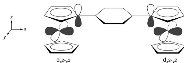
Figure 3. Overlap between the iron 3d orbitals and the 2p_z orbitals of the bridge.
