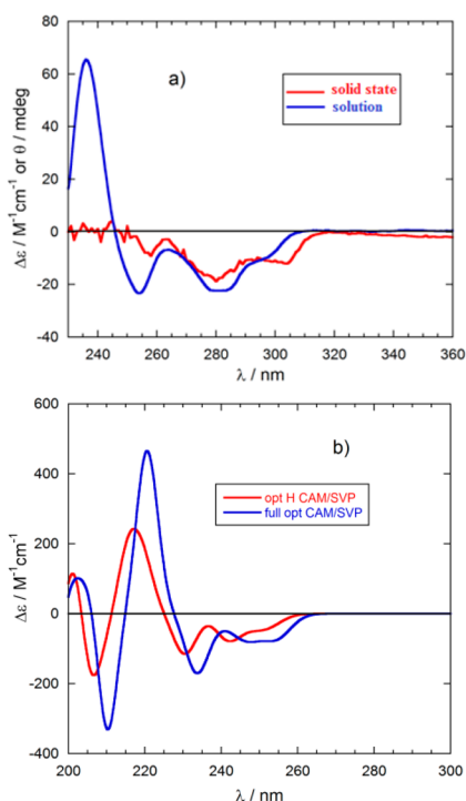
Figure 3. (a) Experimental CD spectra of M -SSS-5a in \text{CH}_2\text{Cl}_2 solution (298 K) and in the solid state; (b) TD-DFT calculated CD spectra of M -SSS-5a on fully optimized and partially optimized (only H atoms) geometries.
