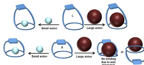
Figure 1. Schematic representation of possible modes of interaction between a long (L) and short (S) strapped calix[4]pyrrole with a small and a large anion.
