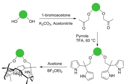
Scheme 1. Schematic Representations of Synthesis of Receptors
