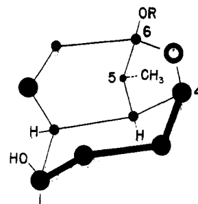
Fig. 2.— \gamma -Lactol structure.
