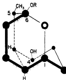
Fig. 1.— \delta -Lactol structure.
