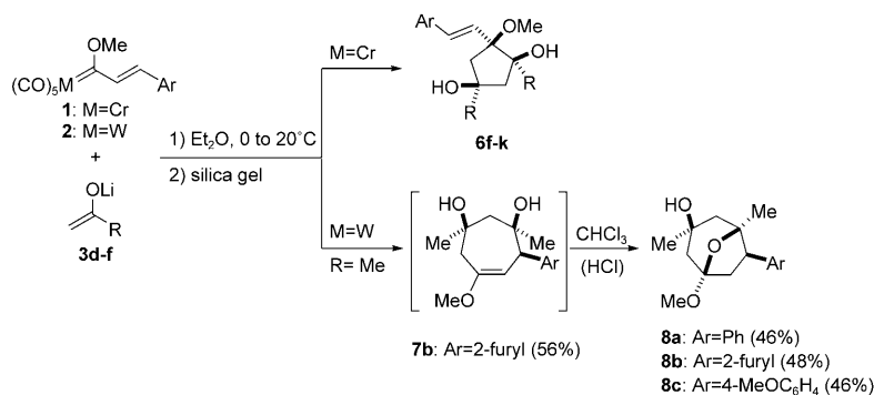
Scheme 2. Reaction of carbene complexes 1 or 2 with alkyl methyl ketone lithium enolates 3d–f to give 1,3-cyclopentanediol derivatives 6f–k , 5-cycloheptene-1,3-diols 7 , and 8-oxabicyclo[3.2.1]octanes 8 .
