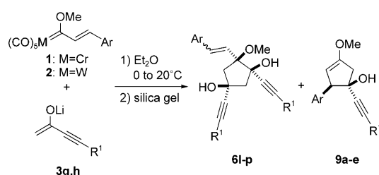
Scheme 3. Reaction of carbene complexes 1 or 2 with alkynyl methyl ketone lithium enolates 3g, 3h to give 1,3-cyclopentanediol derivatives 6l–p and 3-cyclopentenols 9a–e .
