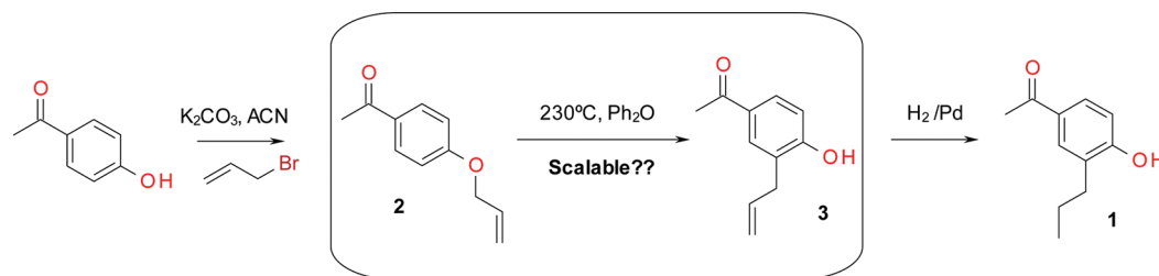
Scheme 1. Synthetic Route
