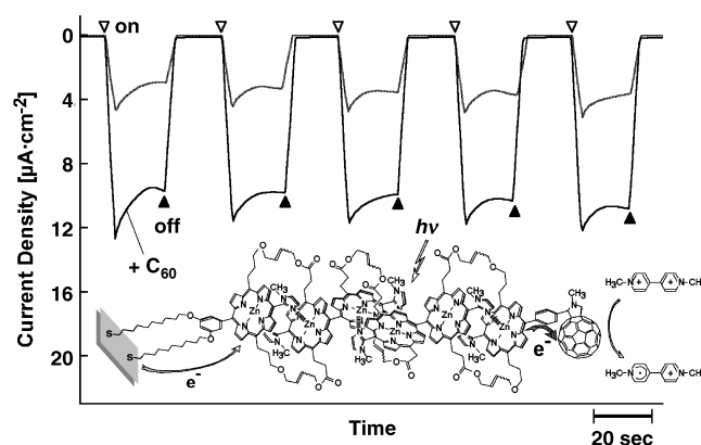
Figure 15. Effect of termination with \text{C}_{60} at the multiporphyrin array on the photocurrent response at -200 mV versus Ag/AgCl.
