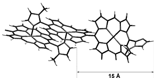
Figure 7. Molecular model of \text{Zn}_2(\text{ImP})_2 coordinating with imidazolymporphyrinatozinc drawn by the molecular mechanics calculation software (Cerius 2 supplied by Accelrys, Ver. 4.6/Force Field UNIVERSAL 1.02). The view omits the allyl side chains for visual clarity.
