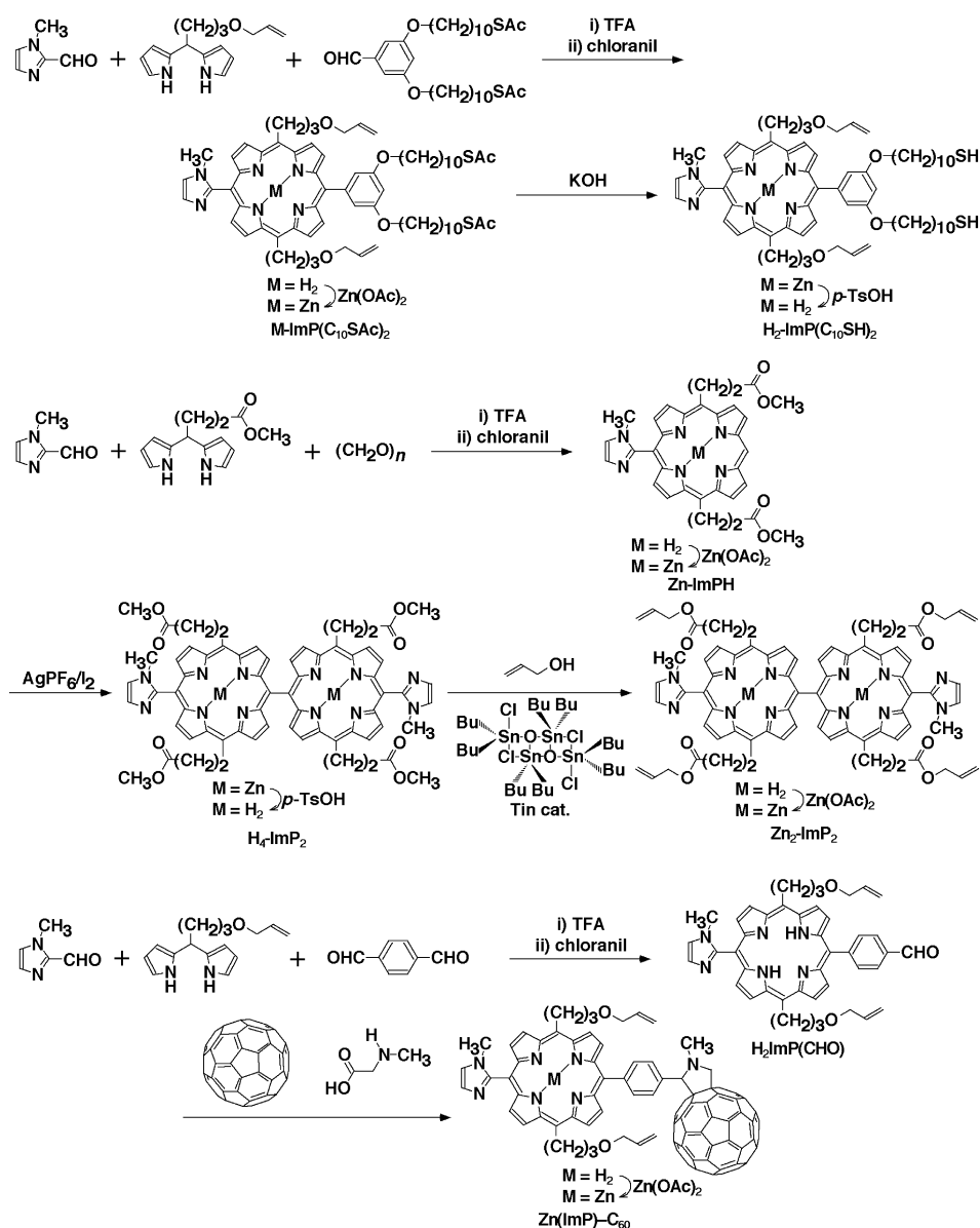
Scheme 3. Synthesis of the imidazolyporphyrins.
