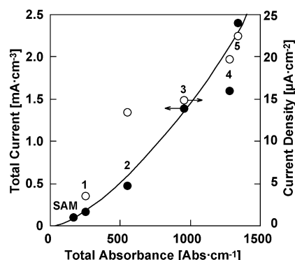
Figure 13. Plots of the photocurrent against the total absorbance at -200 mV (versus Ag/AgCl). The total absorbance was estimated from the integration of the absorption (arbitrary unit) from 350 to 750 nm in wavenumbers ( \text{cm}^{-1} ). The total current density on the left-hand axis ( \bullet ) was calculated from the integration of the current density ( \text{A cm}^{-2} ) in Figure 11 from 380 to 750 nm in wavenumbers ( \text{cm}^{-1} ). The current density on the right-hand axis ( \circ ) was obtained by white light irradiation as shown in Figure 10. The numbers in the figure denote the deposition cycles.
