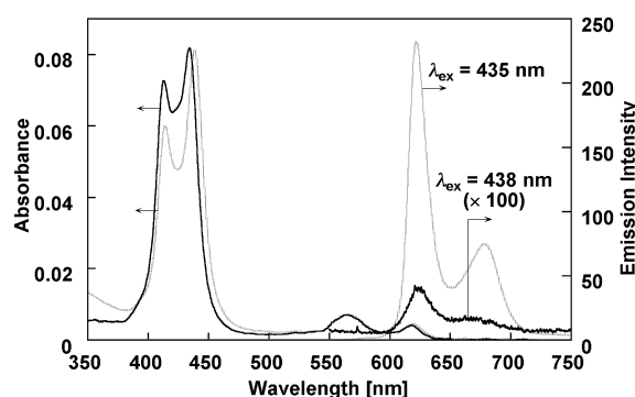
Figure 14. Normalized absorption and emission spectra of \text{Zn}(\text{ImP}) (thin lines) and \text{Zn}(\text{ImP})\text{-C}_{60} (thick lines) in \text{CH}_2\text{Cl}_2 . The fluorescence spectrum was obtained by excitation at the longer Soret band. The fluorescence of \text{Zn}(\text{ImP})\text{-C}_{60} is magnified by 100 times.
