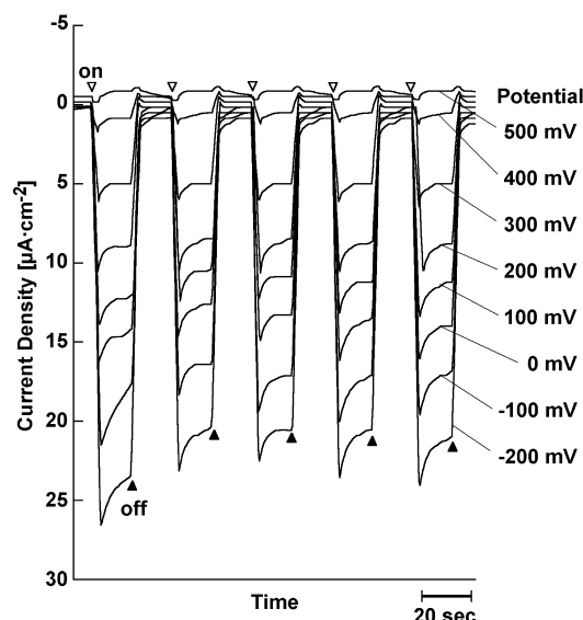
Figure 8. Photoresponse patterns during on/off cycles of white light at various potentials. Conditions: \text{Na}_2\text{SO}_4 (0.1 M) supporting electrolyte and methylviologen (10 mM) electron-carrier in the aqueous system under nitrogen streaming. The \text{Zn}_2(\text{ImP})_2 was accumulated over four deposition cycles.
