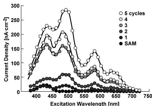
Figure 10. Photocurrent-action spectra of the multiporphyrin on the gold electrode at -200 \text{ mV} versus \text{Ag/AgCl} . The spectra were normalized to a constant light intensity at 174.6 \mu\text{W cm}^{-2} .
