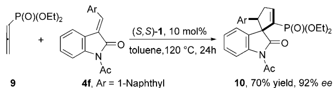
Scheme 4. Stereoselective synthesis of the \alpha -phosphorylated spirooxindole 10 under catalysis by 1 .
