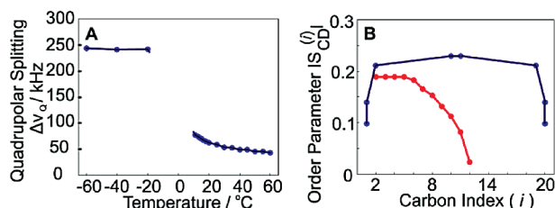
Figure 2. (A) De-Paked quadrupolar splittings ( \Delta\nu_Q ) of [10',11'\text{-}^2\text{H}_2]\text{C}_{20} -BAS-PC as a function of temperature. (B) Order parameters |S_{\text{CD}}^{(i)}| of \text{C}_{20} -BAS-PC (blue) at 25 °C and DLPC (red) at 30 °C as a function of carbon number.
