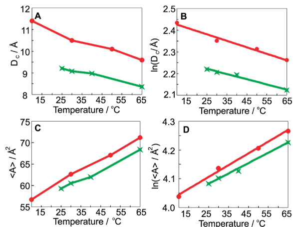
Figure 3. (A) Hydrophobic layer thickness ( D_C ) for [2',2',19',19'\text{-}^2\text{H}_4]\text{C}_{20} -BAS-PC (green) and DLPC (red) as a function of temperature. (B) Natural logarithm of hydrophobic layer thickness, (C) area per lipid, and (D) natural logarithm of area per lipid as a function of temperature.
